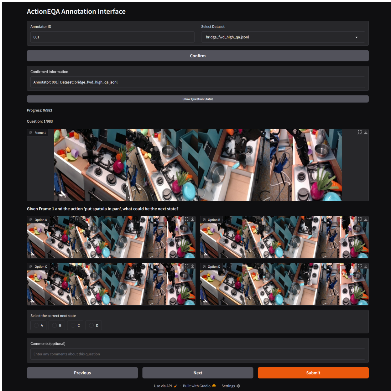
Figure 14: Example of a High-Level State Prediction task on our customized Gradio-based annotation interface for evaluating human performance. In this interface, annotators are presented with a current state image, a high-level goal-oriented action, and four candidate images representing possible next states. Their task is to select the image that best matches the most likely next state.
