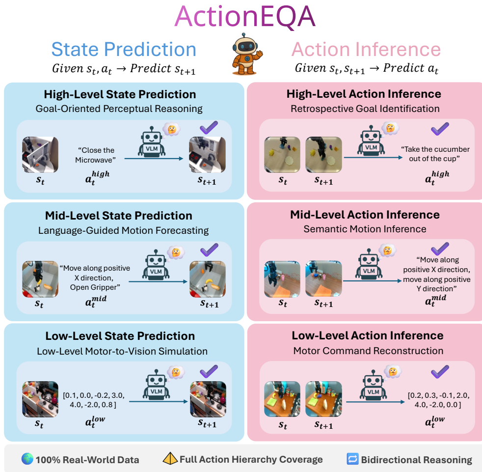
Figure 1: ACTIONEQA assesses the full action hierarchy, from high-level goal-oriented commands to low-level motor commands, through bidirectional action reasoning tasks: State Prediction, which predicts the visual outcome of an action, and Action Inference, which infers the action that caused a visual change.
