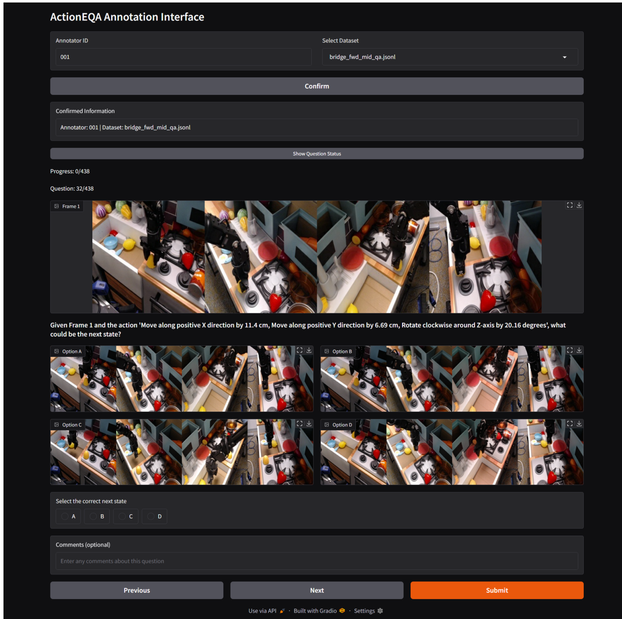
Figure 15: Example of a Mid-Level State Prediction task on our customized Gradio-based annotation interface for evaluating human performance. In this interface, annotators are presented with a current state image, a mid-level natural language motion description, and four candidate images representing possible next states. Their task is to select the image that best matches the most likely next state.
