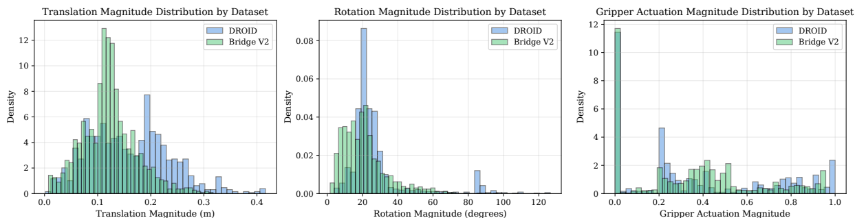
Figure 13: Distribution of low-level action magnitudes across DROID and BridgeData V2 datasets.
