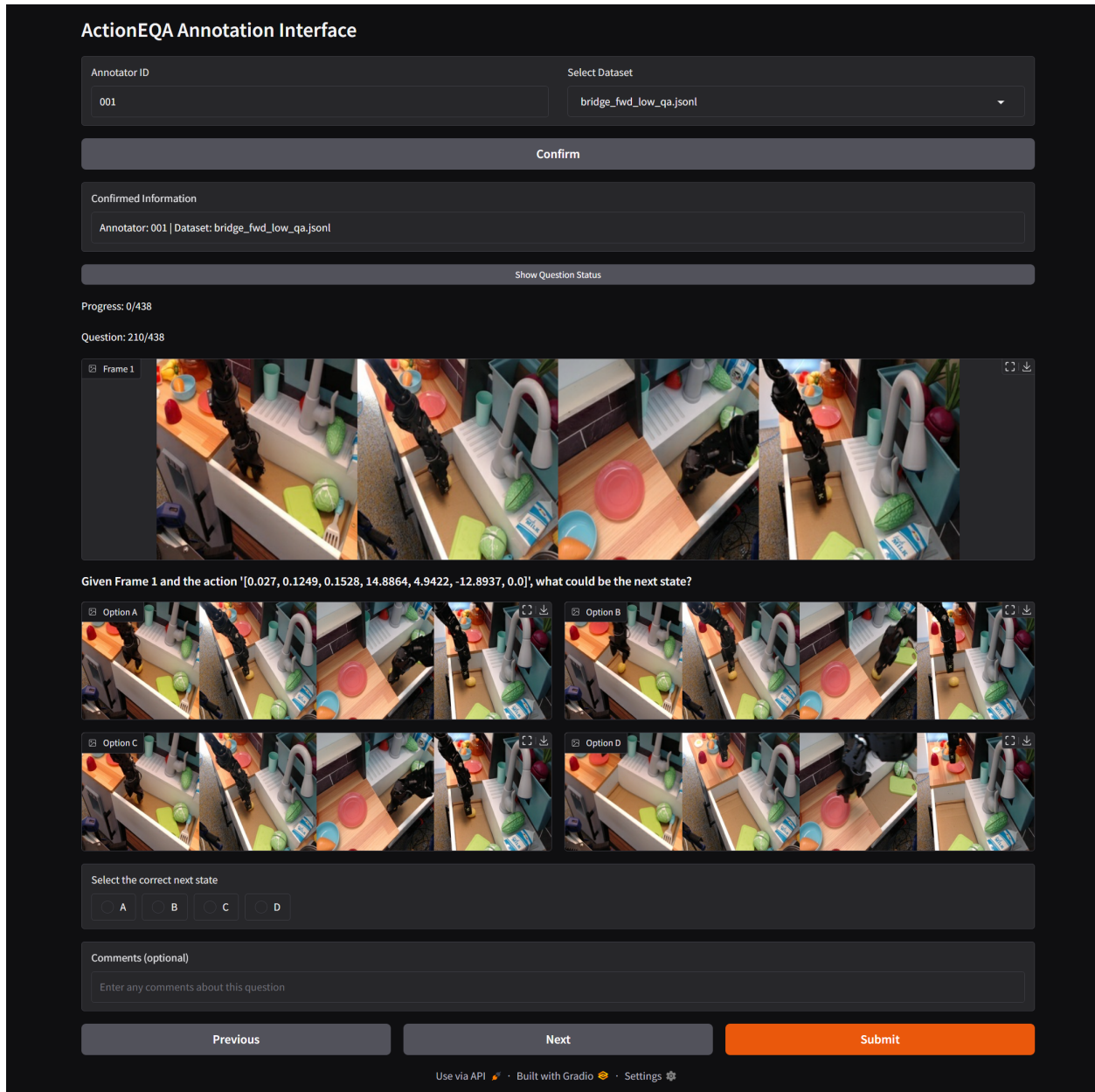
Figure 16: Example of a Low-Level State Prediction task on our customized Gradio-based annotation interface for evaluating human performance. Annotators are shown a current state image, a low-level 7-DoF motor command specifying relative changes in translational motion ( x , y , z ), rotational motion (roll, pitch, yaw), and gripper width, and four candidate images representing possible next states. Their task is to select the image that best corresponds to the most likely next state.
