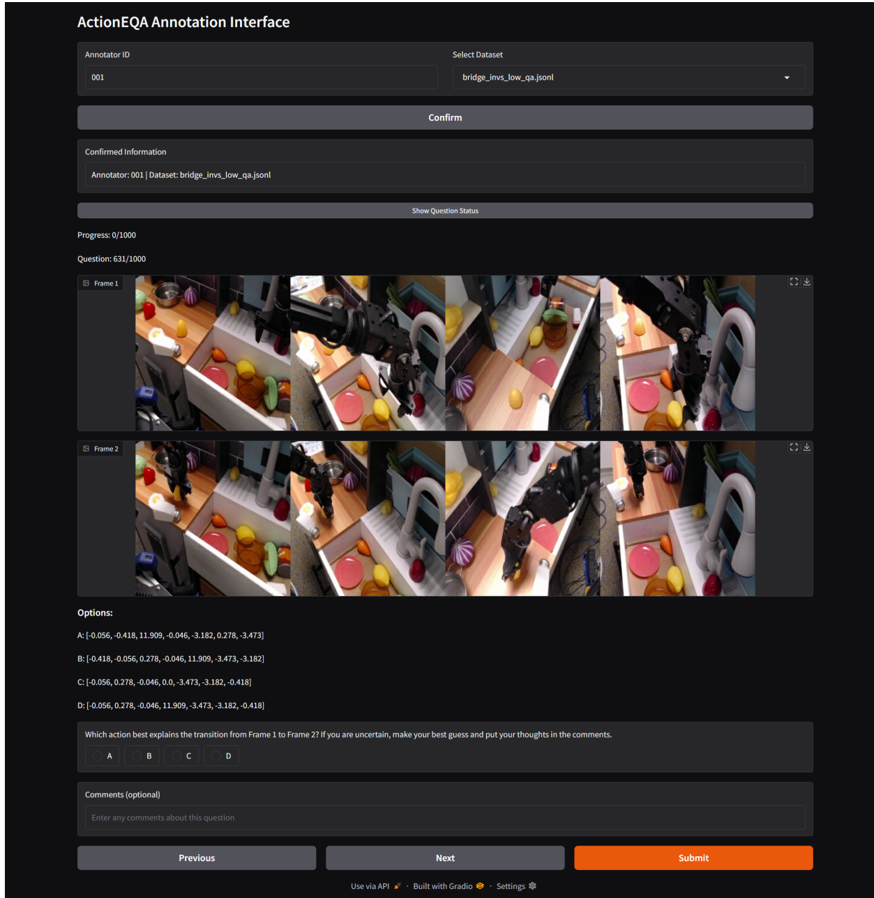
Figure 19: Example of a Low-Level Action Inference task on our customized Gradio-based annotation interface for evaluating human performance. Annotators are presented with a current state image and its resulting next state image, along with four candidate low-level 7-DoF motor commands. Each command specifies relative changes in translational motion (x, y, z), rotational motion (roll, pitch, yaw), and gripper width. The task is to identify the action most likely responsible for the observed transition.
